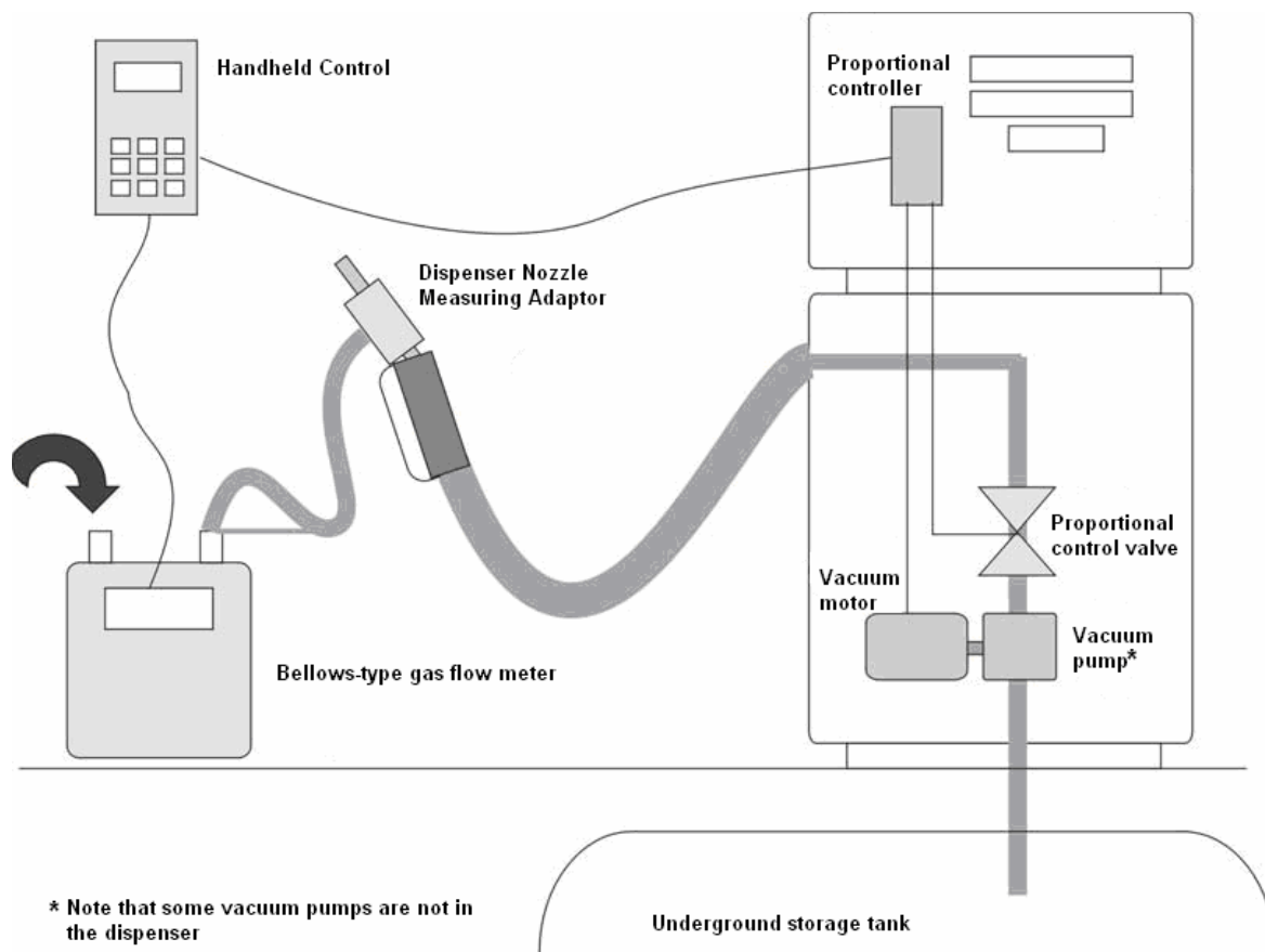
Figure A1: Typical dry method test equipment set up
