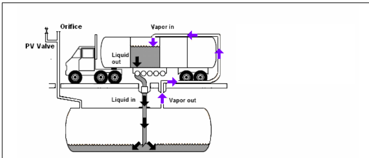
Figure 1: Stage 1 vapour recovery
