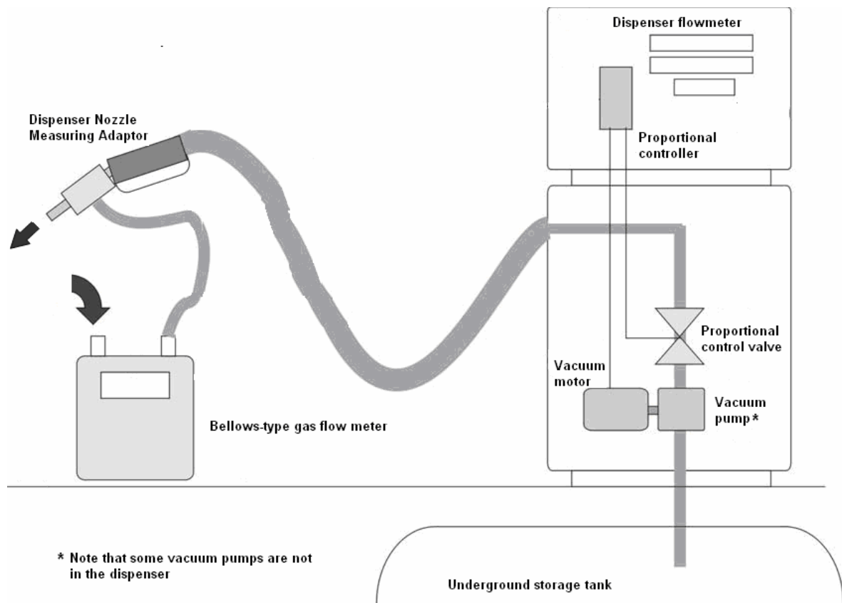
Figure A2: Typical wet method test equipment set up
