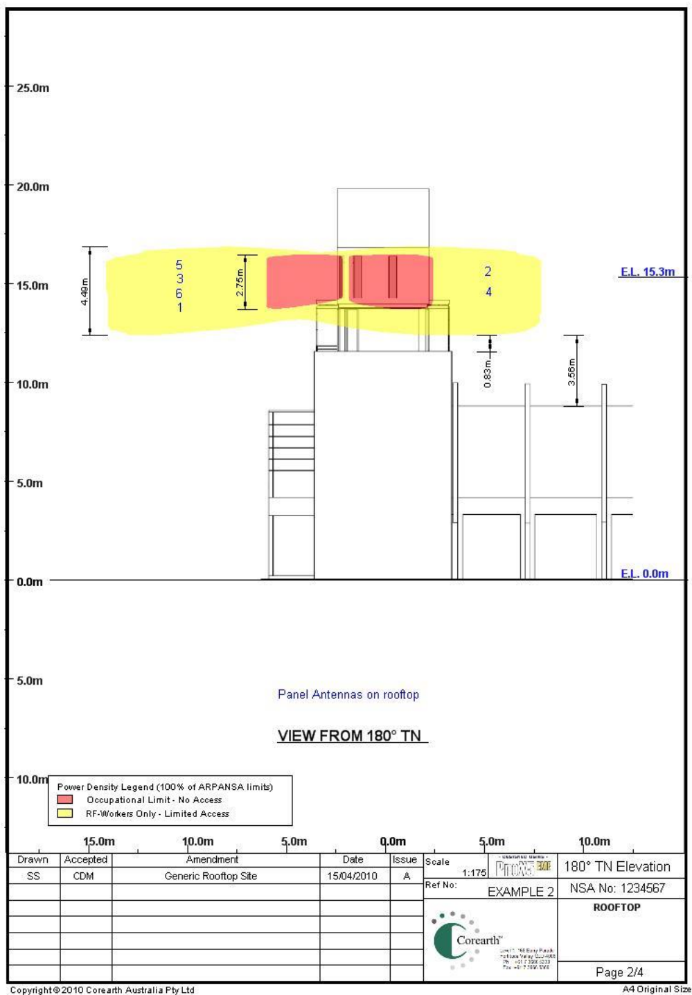
Figure 13: Typical extent of RF field hazard areas of mobile phone base station on roof of building
