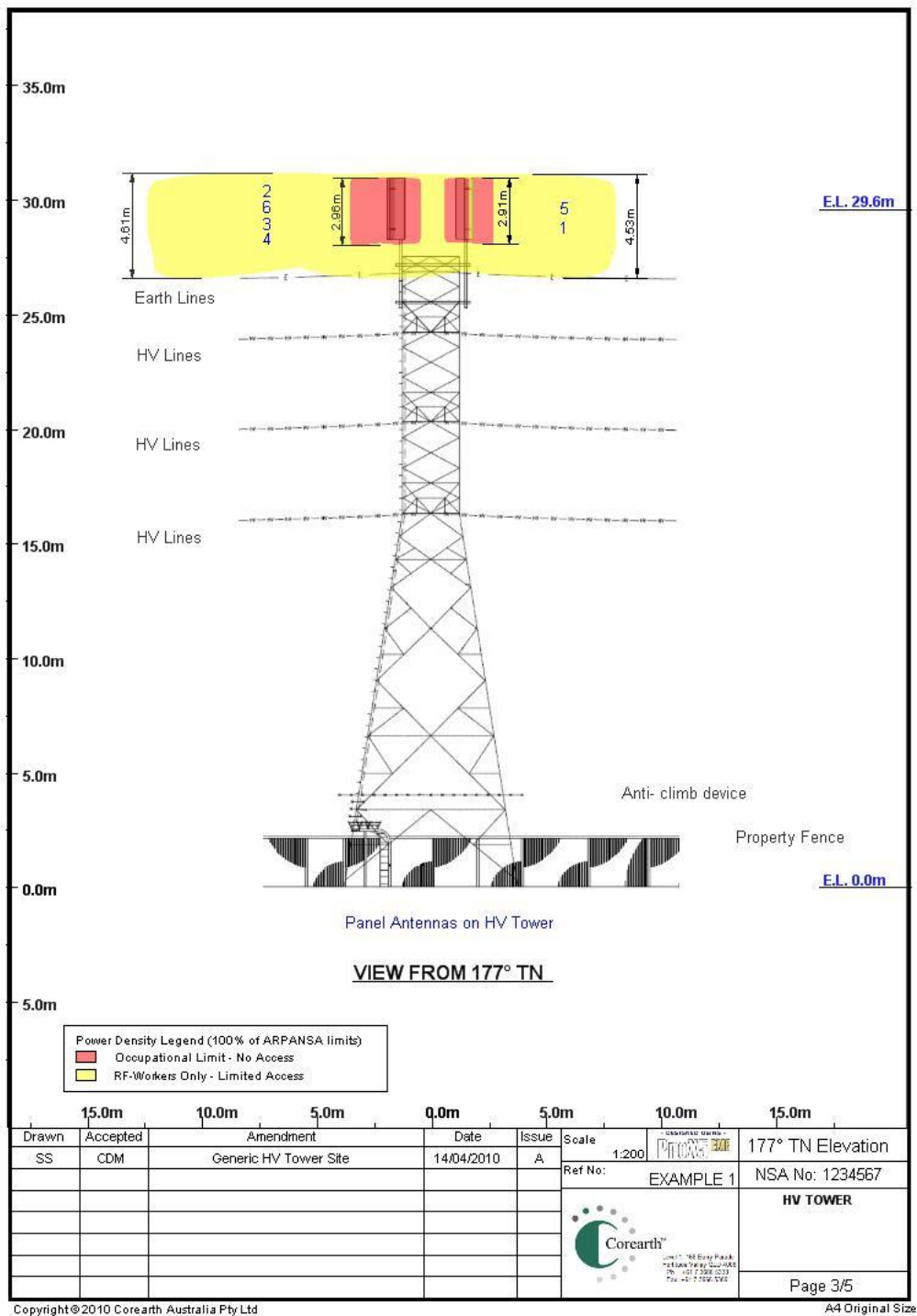
Figure 14: Typical extent of RF field hazard areas of mobile phone base station on electricity tower
